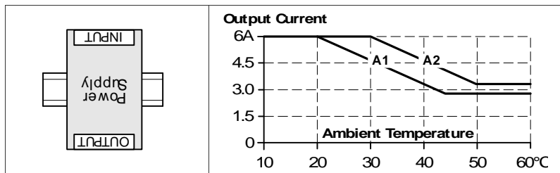
Fig. 23-2 Mounting Orientation B (Upside down)
