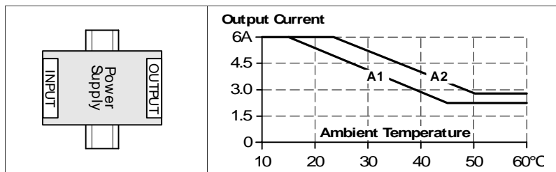
Fig. 23-4 Mounting Orientation D (Horizontal cw)
