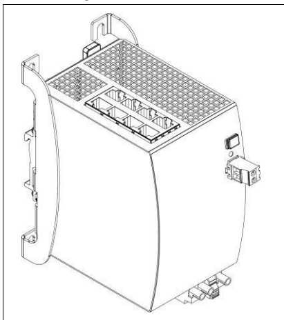
Fig. 22-1 Isometric view
