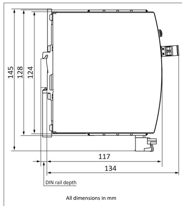
Fig. 21-2 Side view
