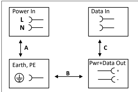
Fig. 18-1 Dielectric strength
