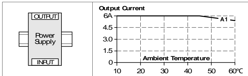
Fig. 23-1 Mounting Orientation A (Standard orientation)
