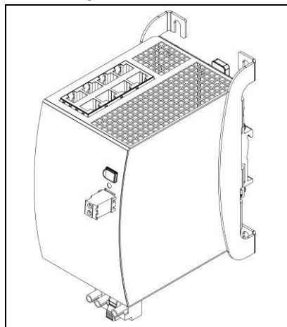
Fig. 22-2 Isometric view
