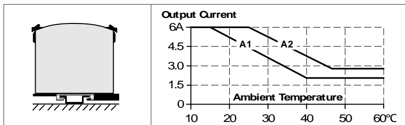
Fig. 23-3 Mounting Orientation C (Table-top mounting)
