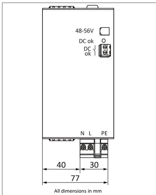
Fig. 21-1 Front view
